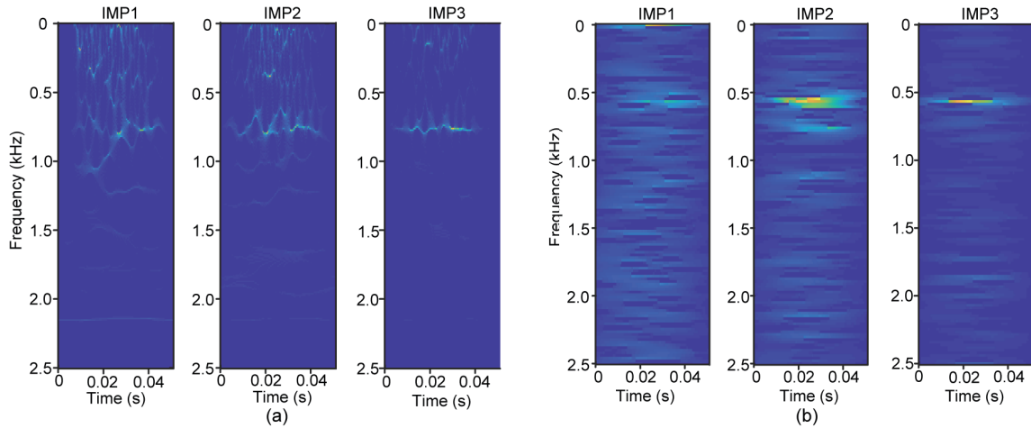
Fig. 2 WSST (a) and FSST (b) time-frequency diagrams of the three different types of HVI sources
